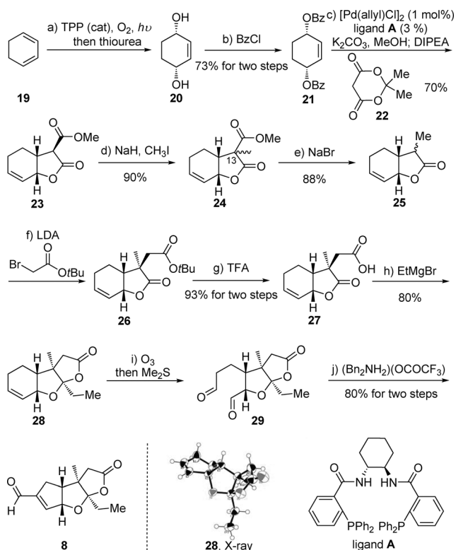
Scheme 4. Reagents and conditions: a) \text{TPP} , \text{O}_2 , h\nu , \text{CCl}_4 , -10^\circ\text{C} then thiourea, \text{MeOH} ; b) \text{BzCl} , \text{Et}_3\text{N} , \text{DMAP} , \text{CH}_2\text{Cl}_2 , RT, 73% for 2 steps; c) [\text{Pd}(\text{allyl})\text{Cl}]_2 (3 mol %), ligand A , 22 , \text{K}_2\text{CO}_3 , \text{MeOH} , THF, 0^\circ\text{C} ; then \text{DIPEA} , 55^\circ\text{C} ; 70%; d) \text{NaH} , \text{CH}_3\text{I} , \text{DMF} , 0^\circ\text{C} , 90%, d.r. (at C13) = 4:1; e) \text{NaBr} , \text{DMF} , 180^\circ\text{C} , 88%, d.r. (at C13) = 1:1; f) \text{LDA} , \text{BrCH}_2\text{CO}_2t\text{Bu} , THF, -78^\circ\text{C} ; g) \text{TFA} , \text{CH}_2\text{Cl}_2 , 0^\circ\text{C} to RT, 93% for 2 steps; h) \text{EtMgBr} , THF/ \text{Et}_2\text{O} (1:1), -78^\circ\text{C} to RT, 80%; i) \text{O}_3 , \text{CH}_2\text{Cl}_2/\text{MeOH} (1:1), -78^\circ\text{C} , then \text{Me}_2\text{S} , -78^\circ\text{C} to RT; j) (\text{Bn}_2\text{NH}_2)(\text{OCOCF}_3) , toluene, 63^\circ\text{C} , 80% for 2 steps. Bz = benzoyl, DIPEA = diisopropylethylamine, DMAP = 4-( N,N -dimethylamino)pyridine, LDA = lithium-diisopropyl amide, TPP = 5,10,15,20-tetraphenyl-21 H ,23 H -porphine. Thermal ellipsoids are shown at 50% probability. [11]
