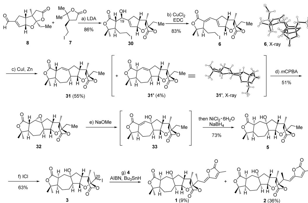
Scheme 5. Reagents and conditions: a) LDA, THF, -78^{\circ}\text{C} , then 8 , 86%, d.r. (at C19) = 17:1; b) \text{CuCl}_2 , EDC, toluene, 80^{\circ}\text{C} , 83%; c) \text{CuI} , \text{Zn} , \text{Pyr}/\text{H}_2\text{O} (1:4), ultrasound, RT, 55% for 31 , 4% for 31' ; d) m CPBA, \text{NaHCO}_3 , \text{CH}_2\text{Cl}_2 , -15^{\circ}\text{C} , 51%; e) \text{NaOMe} , \text{MeOH} , RT; then \text{NiCl}_2 \cdot 6\text{H}_2\text{O} , \text{NaBH}_4 , \text{MeOH}/\text{THF} (1:5), -15^{\circ}\text{C} , 73%; f) \text{ICl} , THF, RT, 63%, d.r. (at C20) = 1.5:1; (g) 4 , AIBN, \text{Bu}_3\text{SnH} , toluene, 4 Å M.S., 100^{\circ}\text{C} , 9% for 1 , 36% for 2 . EDC = 1-(3-dimethylaminopropyl)-3-ethylcarbodiimide m CPBA = m -chloroperbenzoic acid. Thermal ellipsoids are shown at 50% probability. [21]
